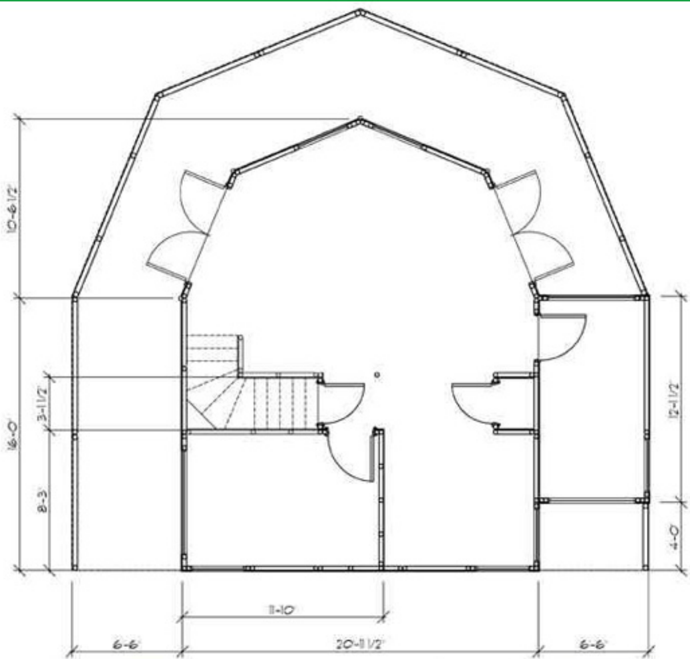
New THAI HALE Floor Plan 670 sq ft interior with loft plus 72 sq ft porch room 480 sq ft deck area
